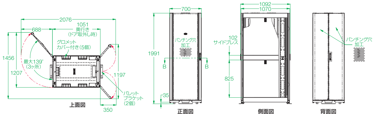
NetShelter SX 42U AR3130
